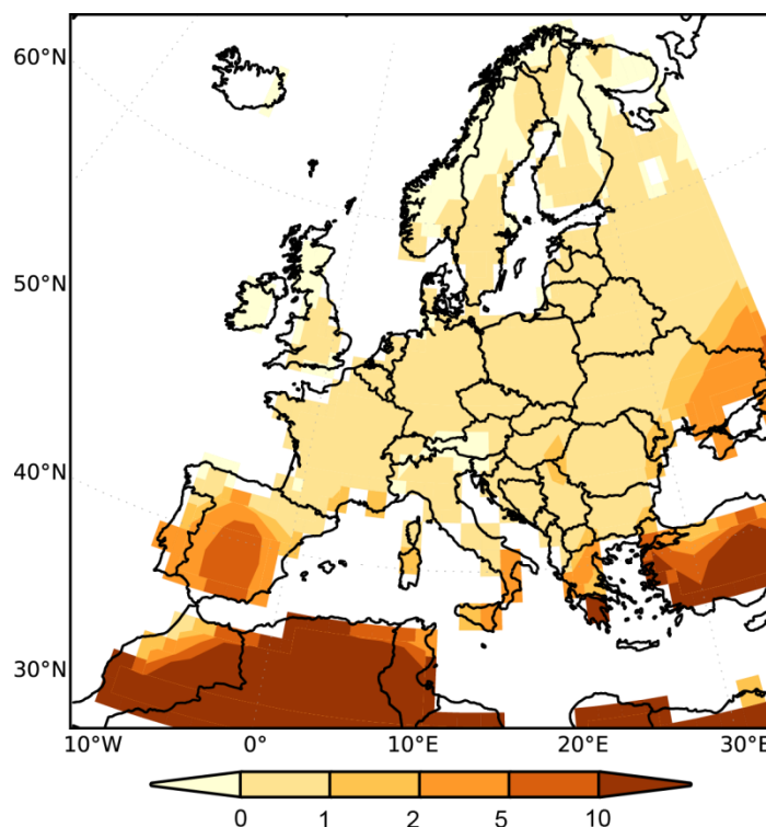
Fig. 13.3. Probability (%) of forest fires, FWI > 45, during the period 1981-2010 based on ERA-Interim data.
