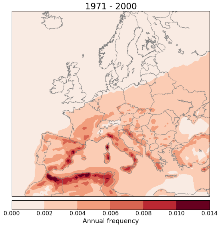
Fig. 14.5. as in Fig. 14.4, but for very large hail (diameter \geq 5 cm).
