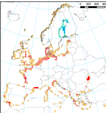
Fig. 6.7. Total area of 100-year coastal flood hazard zones (no flood protection), aggregated to 50x50 km grid, and changes under climate scenarios. Coastal floods
