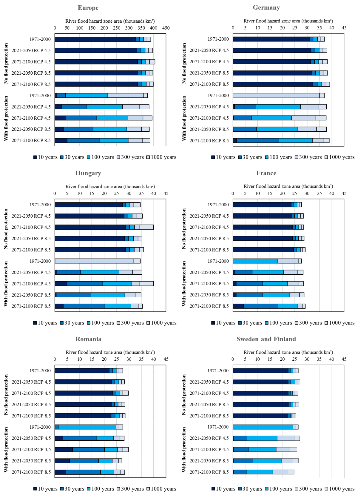
Fig. 7.12. Impact of climate change on river flood hazard zone area, with and without flood protection, for selected countries and Europe within the domain (note different scale for the graph for Europe).
