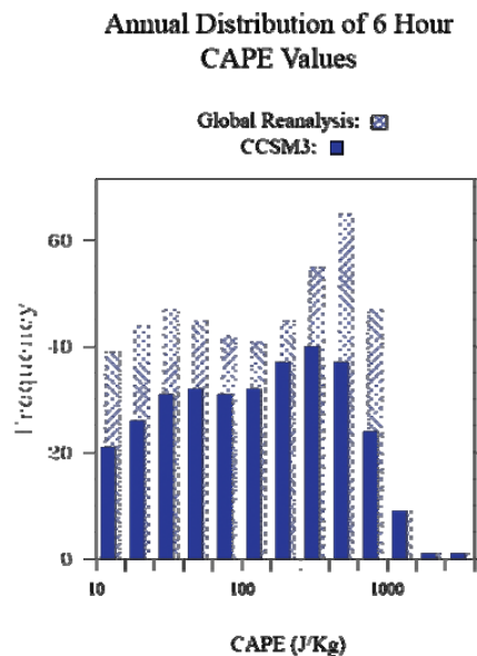
FIG 1. Annual distribution of CAPE values over the North American region normalized by grid point. The solid rectangles are the CCSM3 frequencies and the checkered rectangles are from the reanalysis data.
