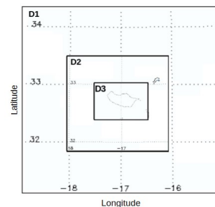
FIG. 2: Horizontal domains used for simulation with grid spacing of 9 km (D1), 3 km (D2) and 1 km (D3).
