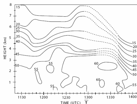
FIG. 2: Time-height representations of data for the storm on 18 August 2004, with contours of reflectivity dBZ. Tornado time (denoted by T) is 1255-1300 UTC. Dashed line is the assumed isolines when the storm is close to the radar.
