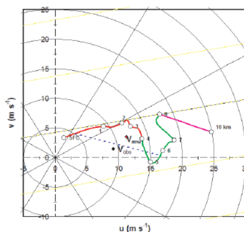
FIG. 1: A hodograph derived from a velocity wind profile derived from the Anjalankoski radar at 1245 UTC just to the north of the supercell track. The observed storm motion is plotted as V_{obs} , V_{mv} is the mean 0-6 km wind.
